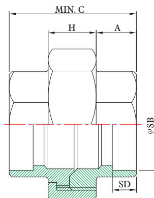
Socket-Weld End
