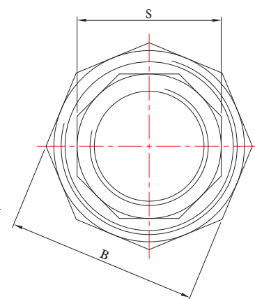
Socket-Weld End
