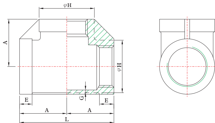
Thread End
