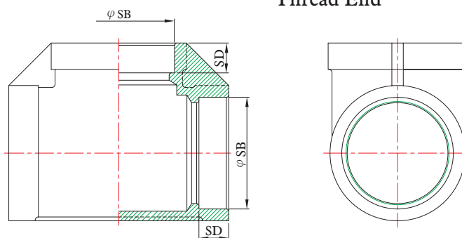
Thread End
