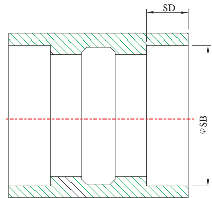
Socket-Weld End
