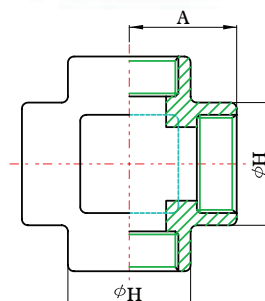
CROSS
