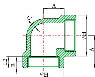
90° ELBOW
