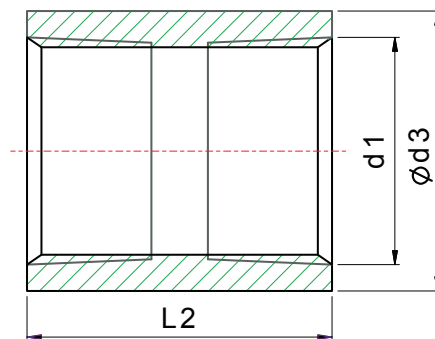
BSPT, NPT
